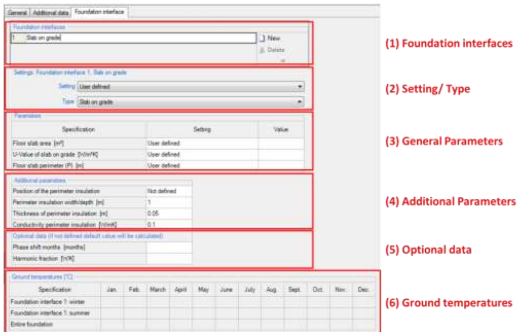
Figure 23: PH Case: Foundation Interface.
