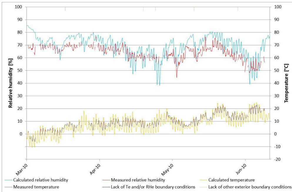
Figure 5. Position B - Outside of the wood studs. Relative humidity: Calculated (blue), measured (red). Temperature: Calculated (yellow) measured (purple). Lack of boundary condition (green/black).
