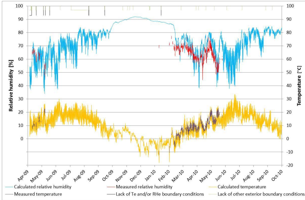
Figure 4. Position B - Outside of the wood studs. Relative humidity: Calculated (blue), measured (red). Temperature: Calculated (yellow) measured (purple). Lack of boundary condition (green/black).
