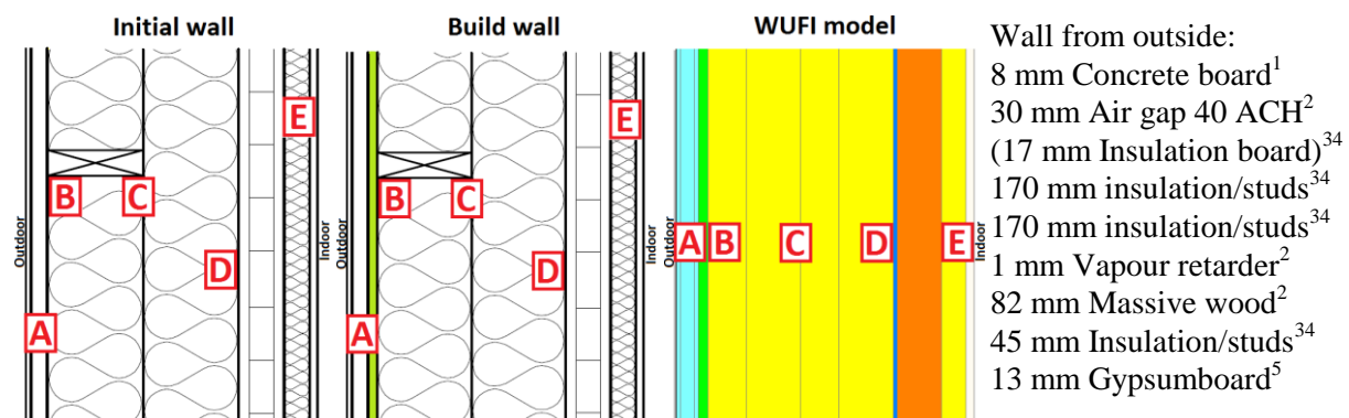
Figure 1. Initial wall without insulation board and Build wall with insulation board (green). Air gap A and measuring positions B to E. Calculation model with insulation board, air gap A and calculated positions B to E. [1. Hedenblad, G. 1996, 2. IBP, 3. IEA Annex 24, 4. Paroc, 5. Krus, M. 1996].
