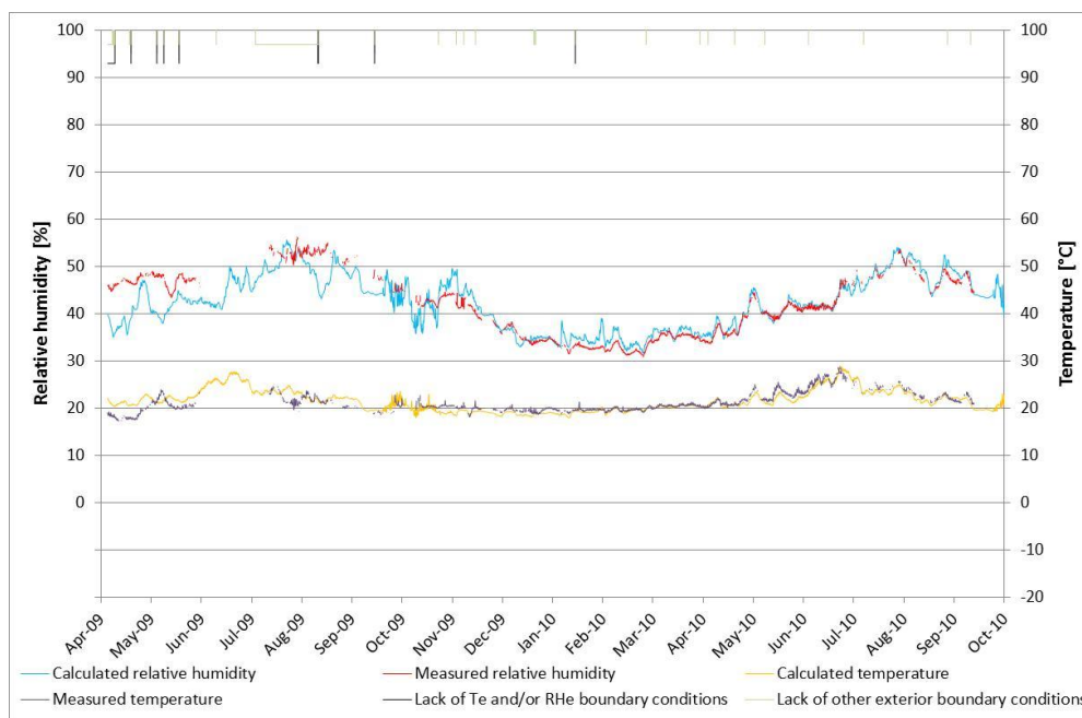
Figure 8. Position E - Installation layer on the warm side of the vapour retarder. Relative humidity: Calculated (blue), measured (red). Temperature: Calculated (yellow), measured (purple). Lack of boundary condition (green/black).
